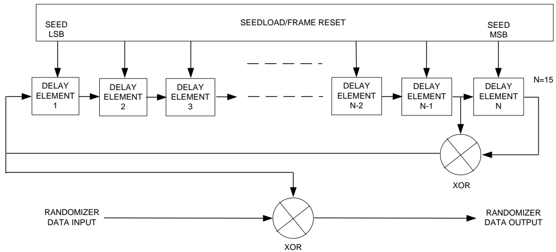
Figure 6–8 - Scrambler Structure
