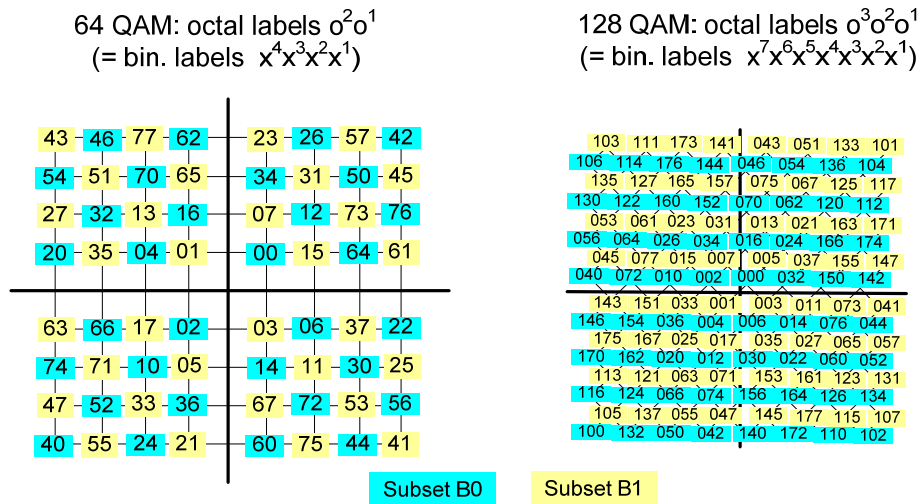
Figure 6-28 - 64-QAM and 128-QAM TCM Symbol Mapping 10
