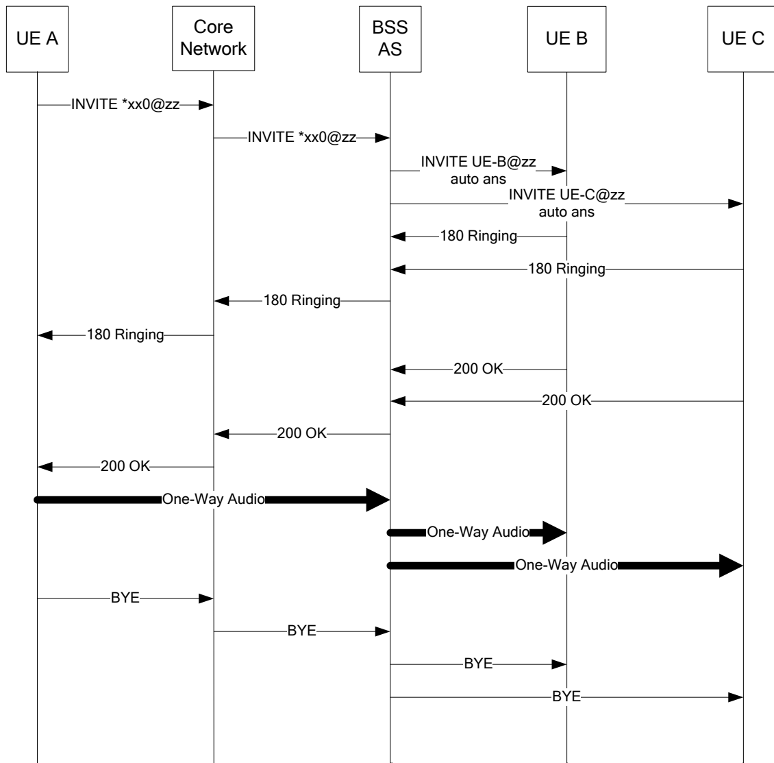
Figure 15 - Loudspeaker Paging
